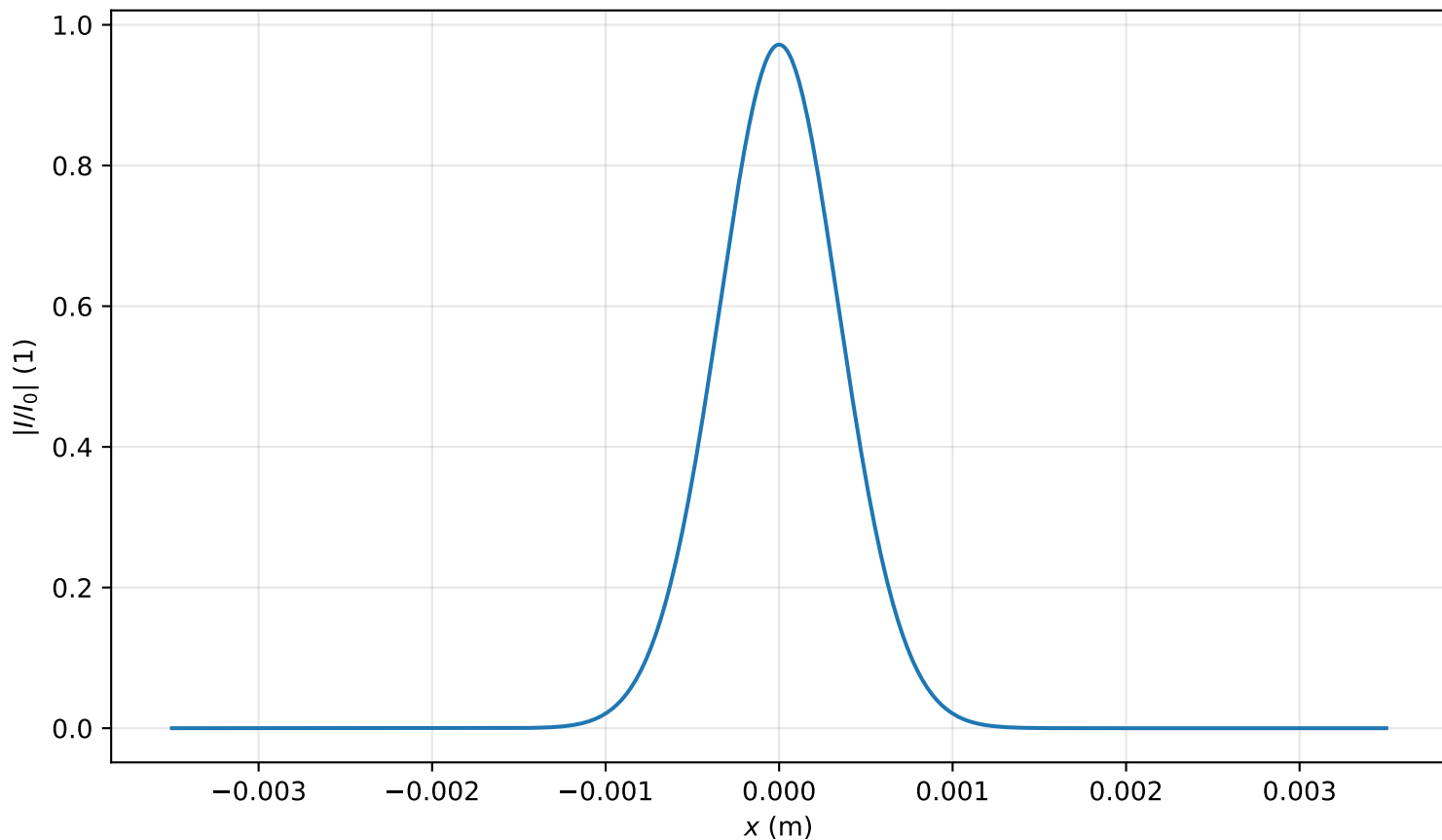
Intensity profile I(x, y = 0, z = 0.557m)/I_0 , P_{in}=0.2P_{cr} , artificial time
